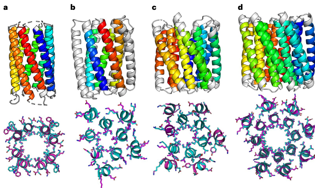
Fig. 4 | Structural characterization of five-helix, six-helix and eight-helix targets. a–d , Top, X-ray crystal structures of sc-apCC-8 at a 2.0-Å resolution (PDB ID, 8QAF) ( a ), sc-CC-5 at a 1.9-Å resolution (PDB ID, 8QKD) ( b ), sc-CC-6-95 at a 2.8-Å resolution (PDB ID, 8QAG) ( c ) and sc-CC-8-58 at a 2.35-Å resolution (PDB ID, 8QAH) ( d ). Coiled-coil regions identified by Socket2 (ref. 72) (packing cutoff,
